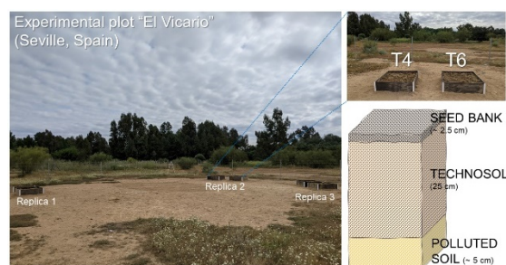
Fig. 1 – Experimental plot and scheme of the rehabilitation system based on Technosols.
